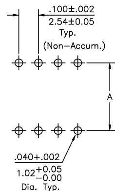
Recommended P.C.Board Hole Layout
